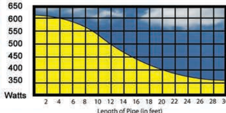
Equivalent light output for straight length of 330mm (13") SunScope (under full sun Summer conditions)
